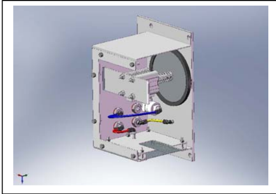
A Typical MotorPurge CLAPS Relief Valve
